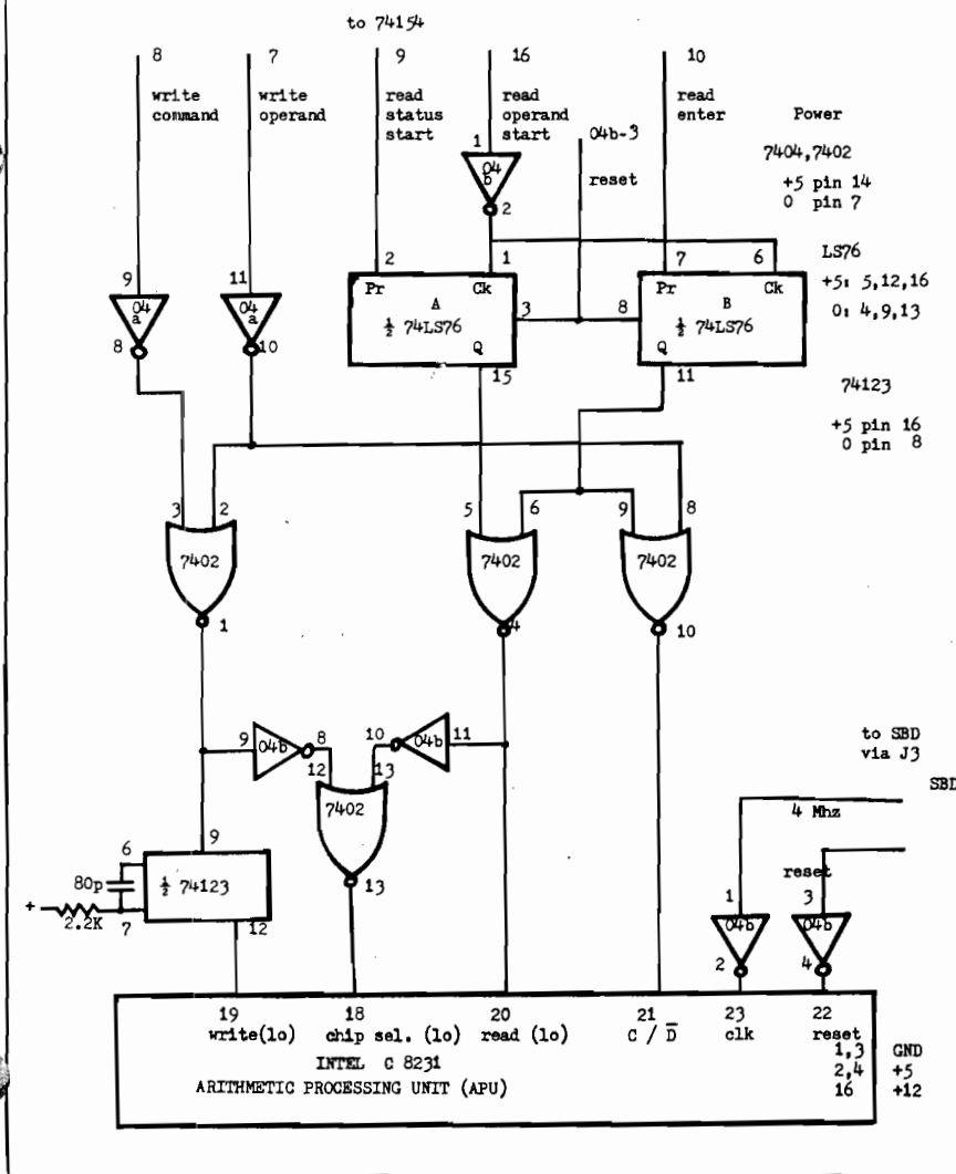
Figure 4: Arithmetic Processing Unit Control
