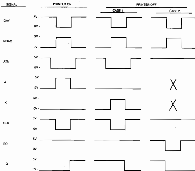
Figure 6: Timing diagram associated with the interface circuit in figure 5.
